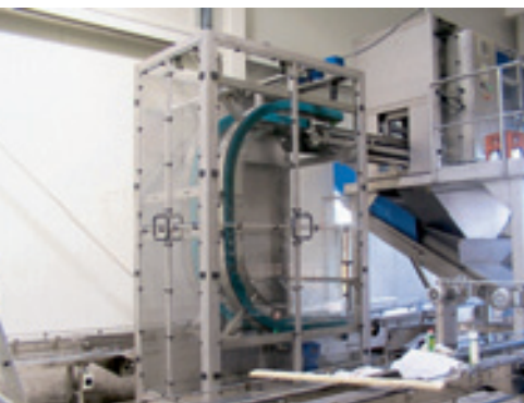
Kastenwender PET-Cycle
